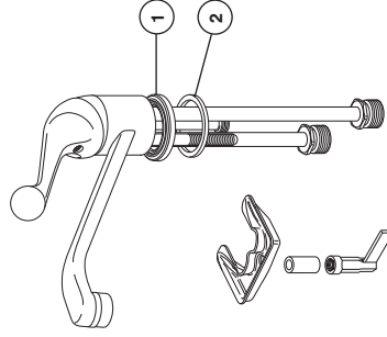
Single Hole Mount 101LF-WF, 175LF-WF & 570LF-WF
