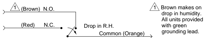
Figure 2 HC-101, HC-101-770, and HC-201 Switch Action and Terminal Identification.
