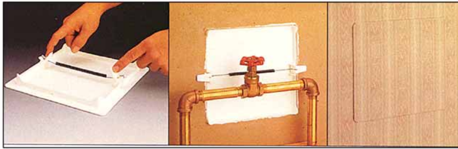
Pull spring-loaded clips into vertical position. Clips clamp against wall when panel is inserted.
