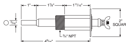
EL1214-P - 3/4" NPT
