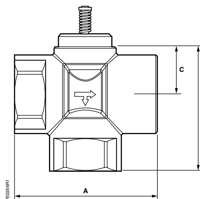
Three-Way Zone Valve Body Dimensions
