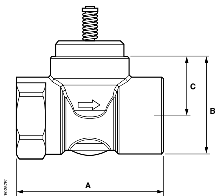
Two-Way Zone Valve Body Dimensions
