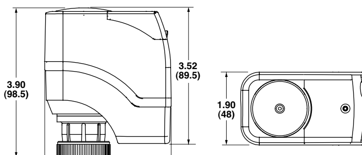
Service Envelope for Two-Way Valve Assembly
