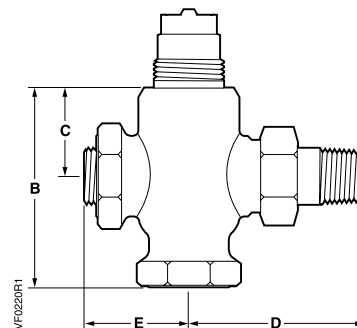
Angle Female by Union Male (AFxFUM)
