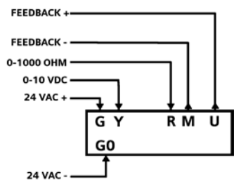
SQS65/65.5 Actuator
