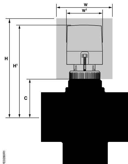
Three-Way Valve Assembly Service Envelope
