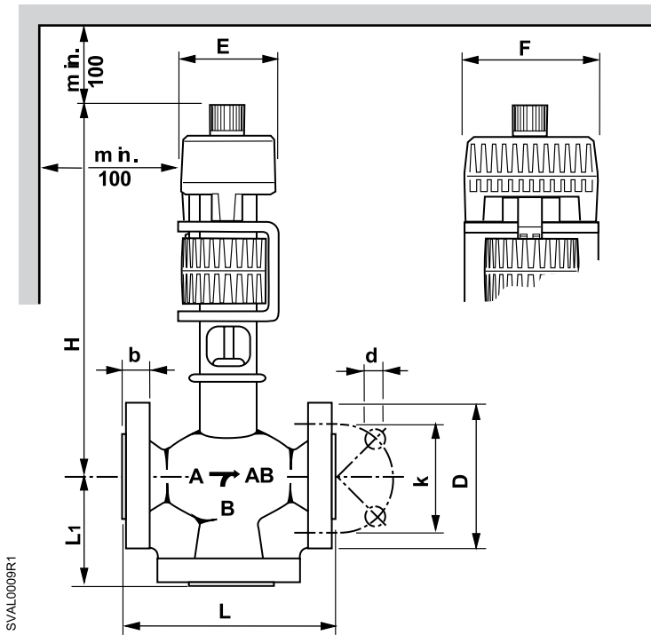
Dimensions shown in inches (mm).
