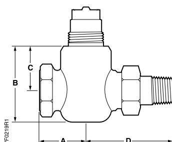
Female NPT by Union Male (FxFUM)
