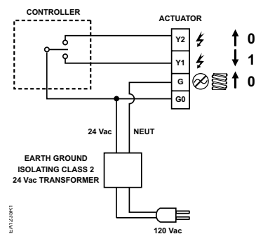
Spring Return (Hot Switching)
