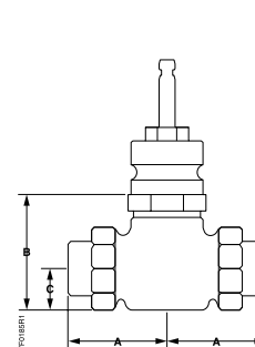
Union Female by Union Female (UFxFUF)
