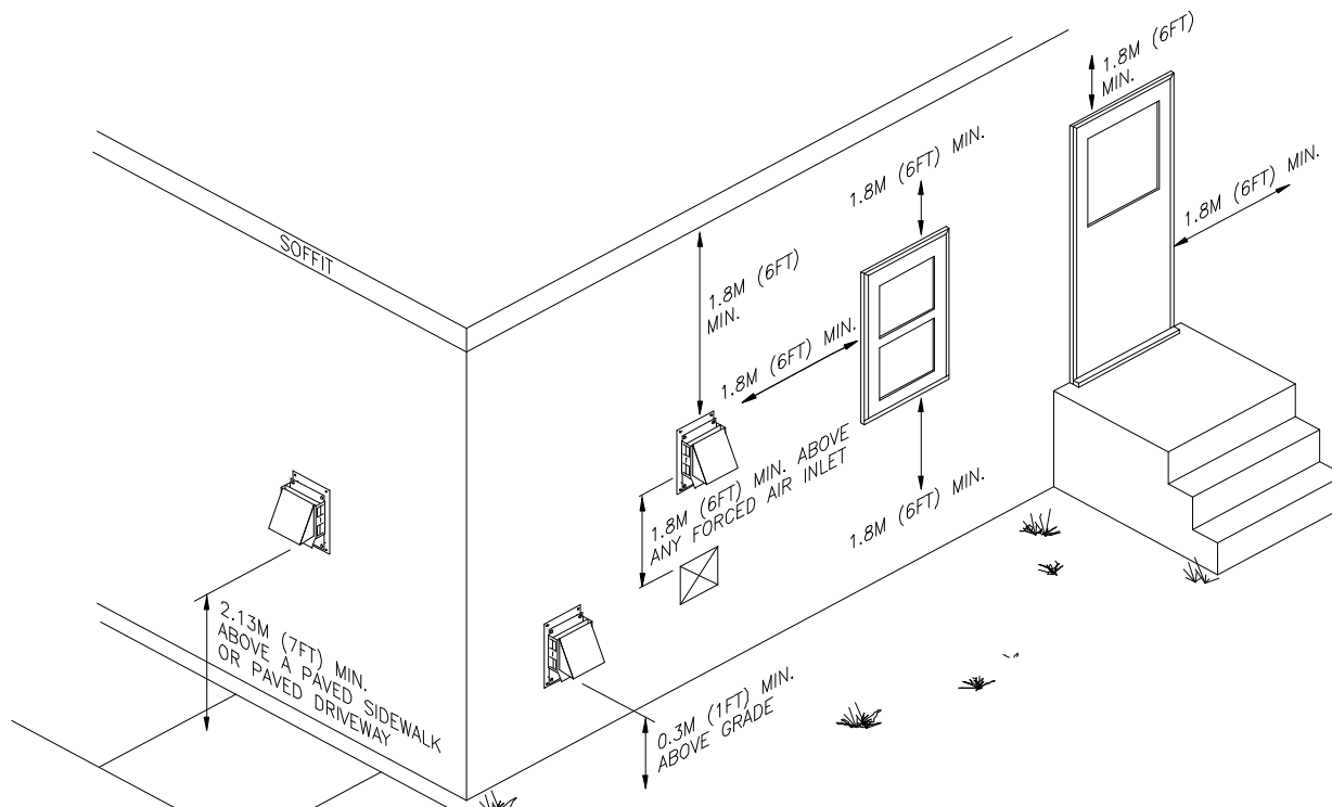
POWER VENTER INSTALLATION
