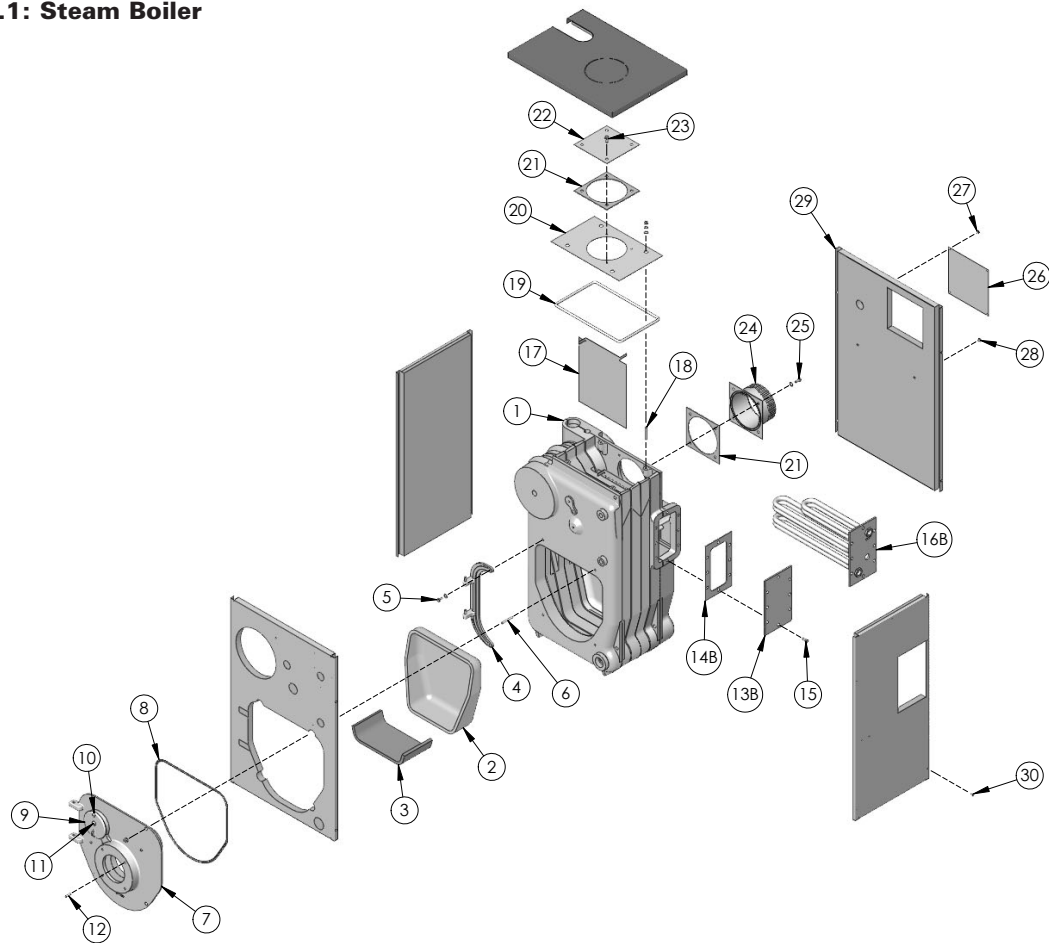
Figure 8.1: Steam Boiler
