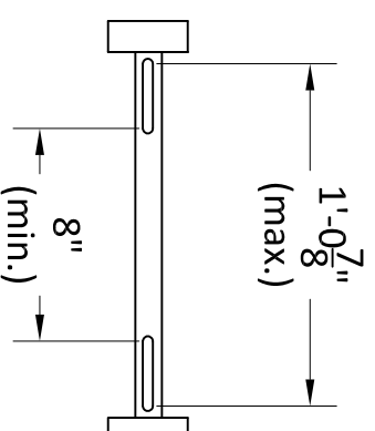
Side View - Expanded
