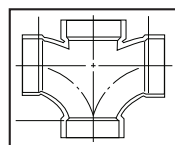
Double Sanitary Tee / Sanitary Cross
