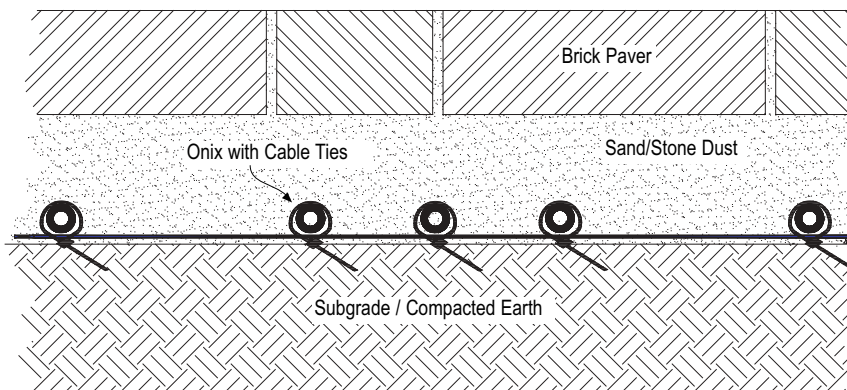
Typical Snowmelt Brick Paver with Cable ties.
