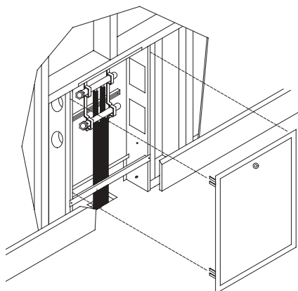
Metal Manifold Enclosure located in wall.
