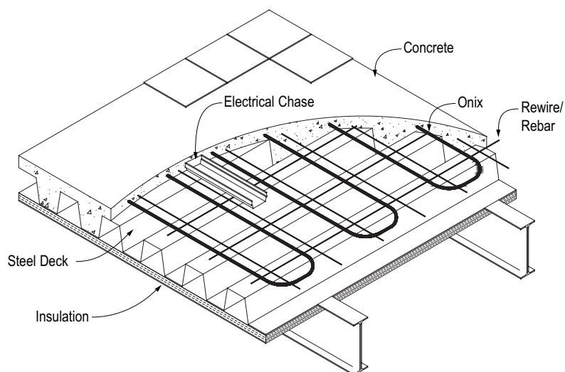
Typical Slab over Steel Deck application. Insulation board is usually installed below the steel deck, minimum 1" thick.
