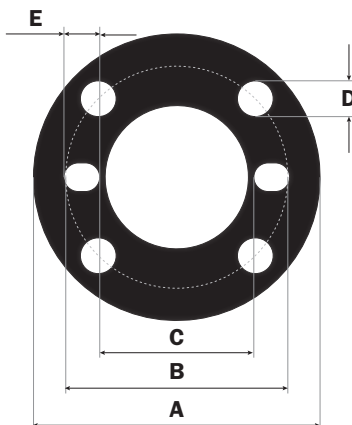
RF375 FLANGE
