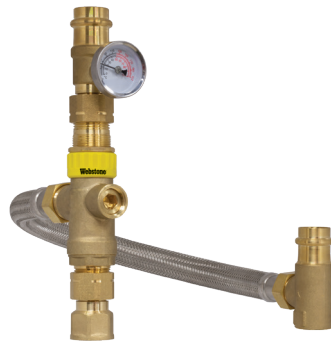
WATER HEATER TEMPERING VALVE W/ TEMPERATURE GAUGE Forged DZR Brass Valve w/ 18" Flex Hose Connector & Integral Check Valves • Outlet Temperature Range 86°-120°F
