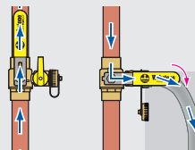
Normal Operation System Purging
